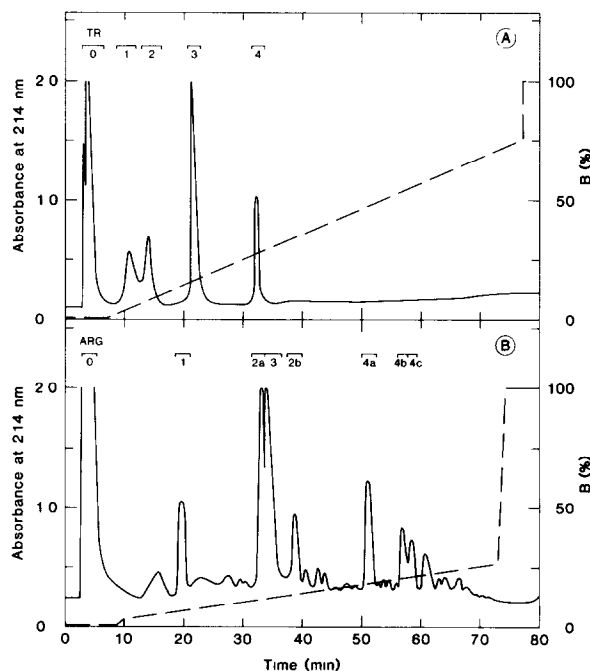
Fig.2. Reversed-phase chromatography on an HR 5/5 Pep RPC (C 2 /C 18 ) column at a flow rate of 0.5 ml/min. Elution was performed with a 80 min gradient from 0 to 25% B, or from 0 to 75% B; solvent A, 0.1% (v/v) trifluoroacetic acid in water; solvent B, 80% (v/v) acetonitrile–0.1% (v/v) trifluoroacetic acid; (A) TR fragments obtained from tryptic digestion of intact protein; (B) ARG fragments obtained from tryptic digestion of lysine-blocked protein.
